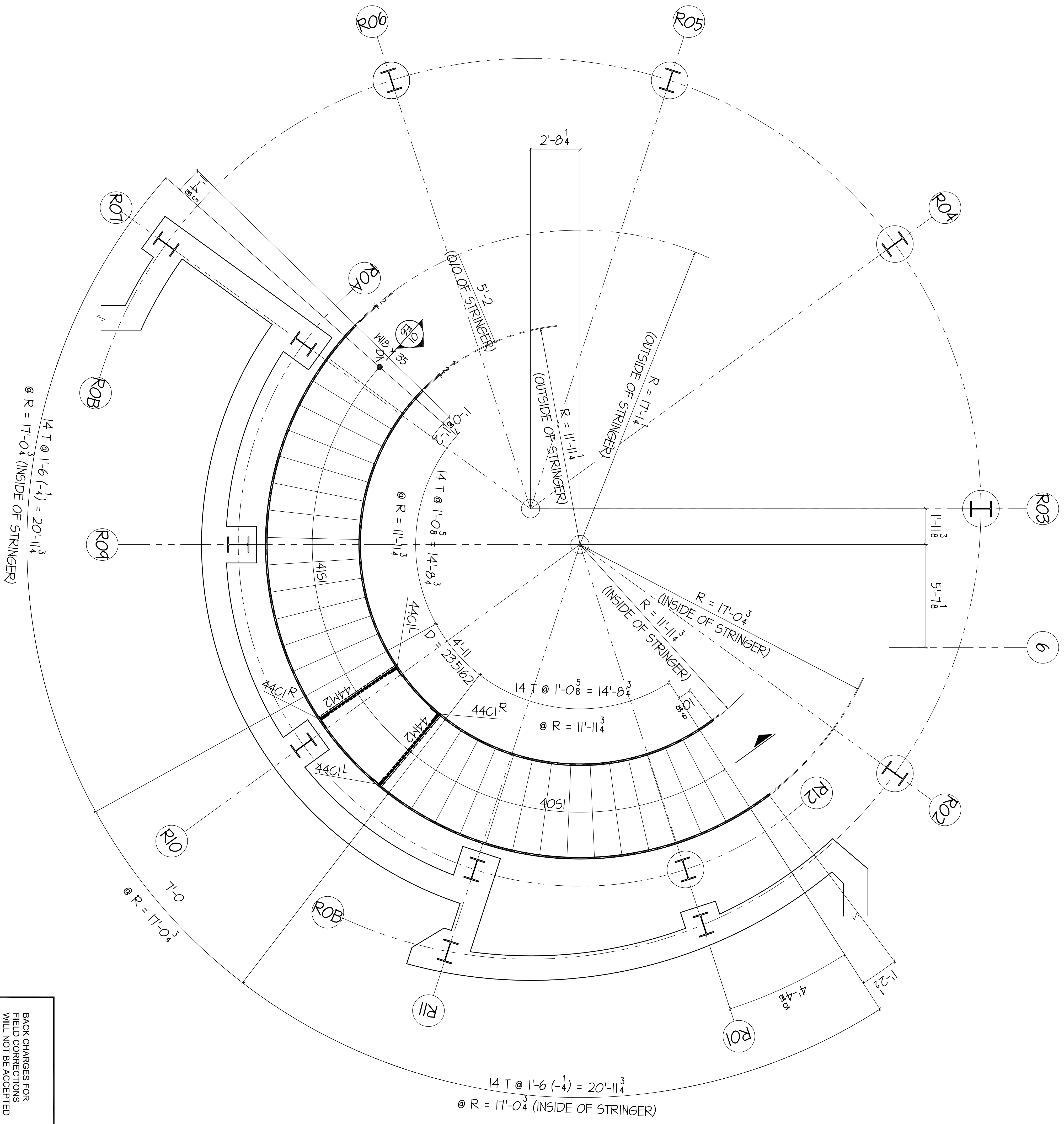
ROTUNDA STAIR PLAN @ STREET LEVEL
